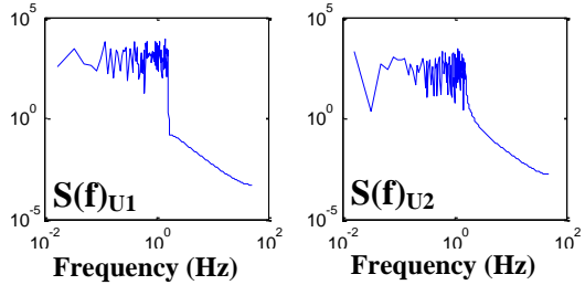
Figure 5. Spectral Analysis of Inlet Velocity Profile
