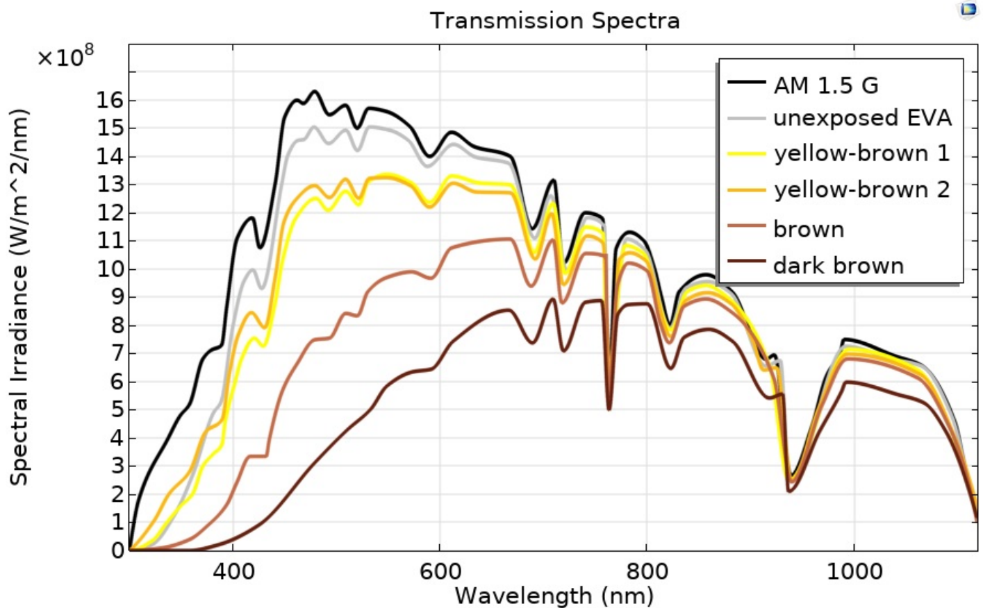
Figure 2 : Transmission spectra at different levels of yellowing, data taken from [3].
