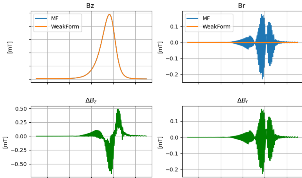
Figure 1 : Results of computed magnetic flux B at the axis. Top left: B_z ; top right: B_r ; bottom left: difference of B_z between MF and weakform; bottom right: difference of B_r between MF and weakform simulation.
