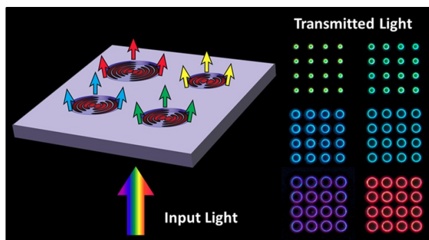
Figure 1: Figure 1. (left) Schematic cartoons showing light shining on, forming surface plasmon drumhead modes, and transmitting through arrays of plasmonic halo structures. (right) Transmission optical microscope images of plasmonic halos with different geometries under white light illumination.
