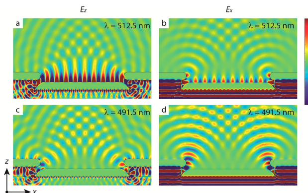
Figure 2: Figure 2. Cross-section views of electric field profiles under x-polarized bottom illumination. (a) E_z profile at resonance (512.5 nm) shows a strong SPP standing wave (cavity mode). (b) E_x at the same wavelength shows weak far-field coupling. (c) E_z profile off resonance (491.5 nm) shows no SPP cavity mode. (d) E_x profile at the same condition shows strong far-field coupling. All four profile maps are on the same linear color scale, from -0.25 to 0.25 V/m, as shown at right.
