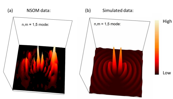
Figure 3: Figure 3. (a) 3 dimensional plot of electric field intensity profile inside a circular plasmonic halo cavity obtained by near-field scanning optical microscopy. (b) 3 dimensional plot of simulated electric field intensity profile within a bounded circular cavity, with light color meaning high and dark color meaning low intensities.
