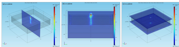
Figure 2: A finite element analysis shows the transmission property of MDSs in (a) y-z plane, (b) z-x plane, and (c) x-y plane
