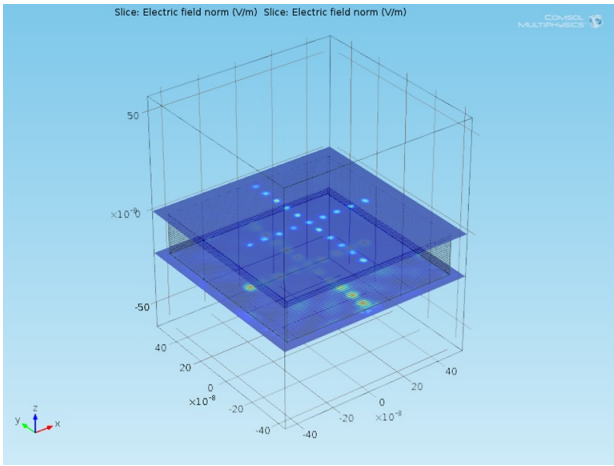
Figure 3: A finite element analysis shows the dipole array can be resolved on the proposed nanostructure
