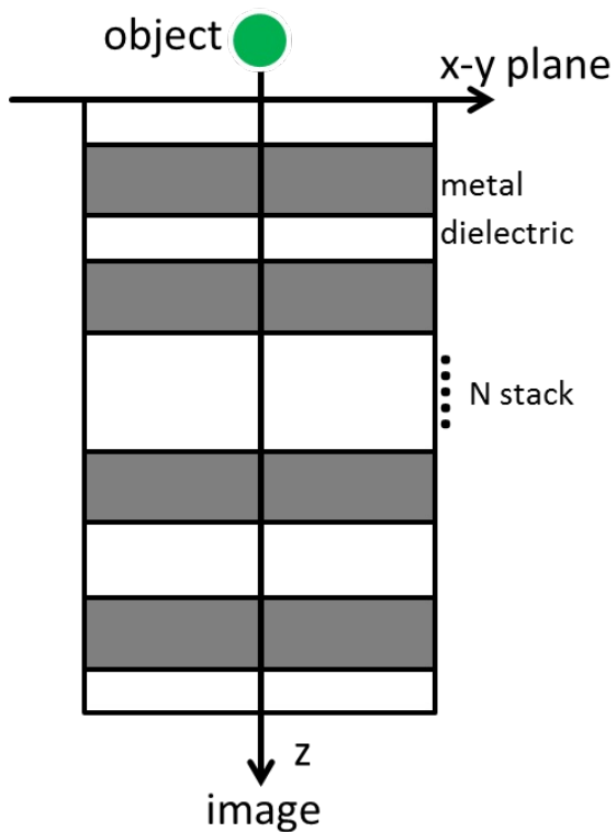
Figure 1: Schematic configuration for the layered metal-dielectric stacks
